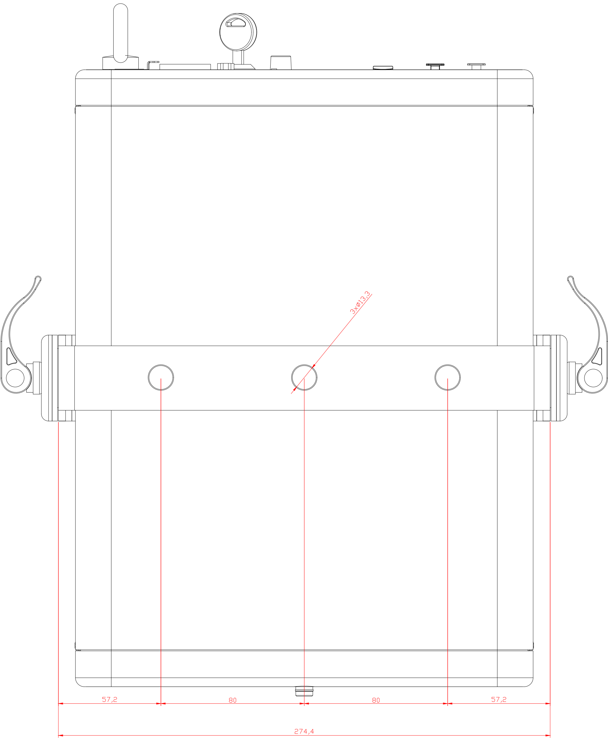
TOP VIEW
