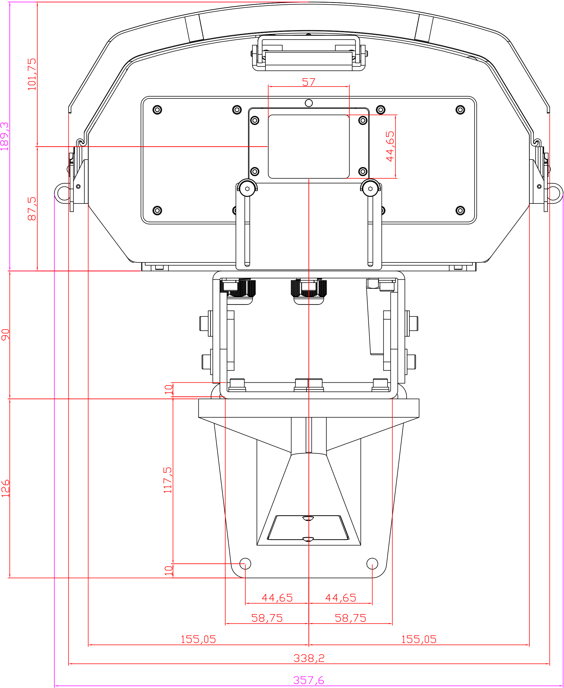
FRONT VIEW
