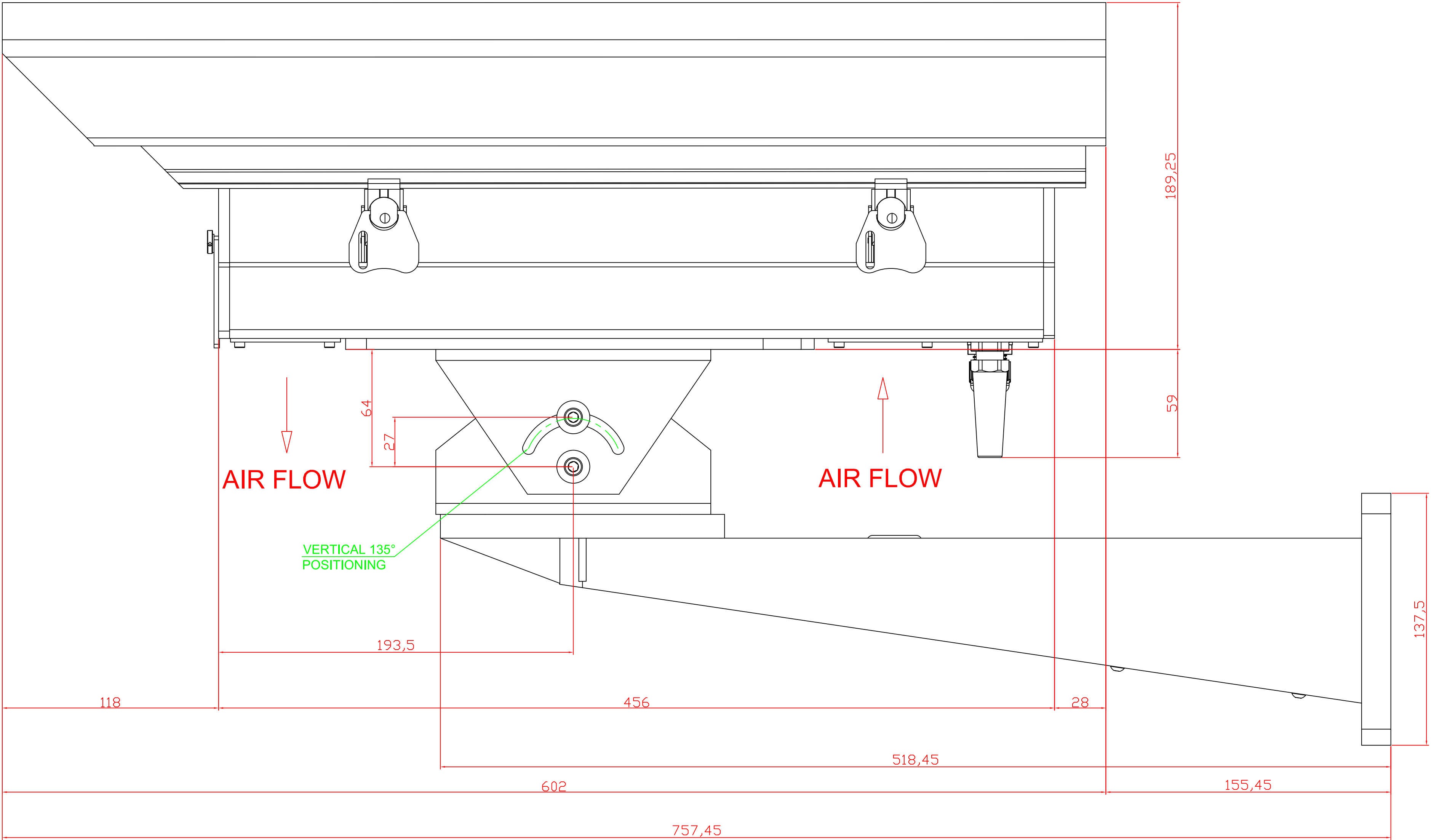
SIDE VIEW
